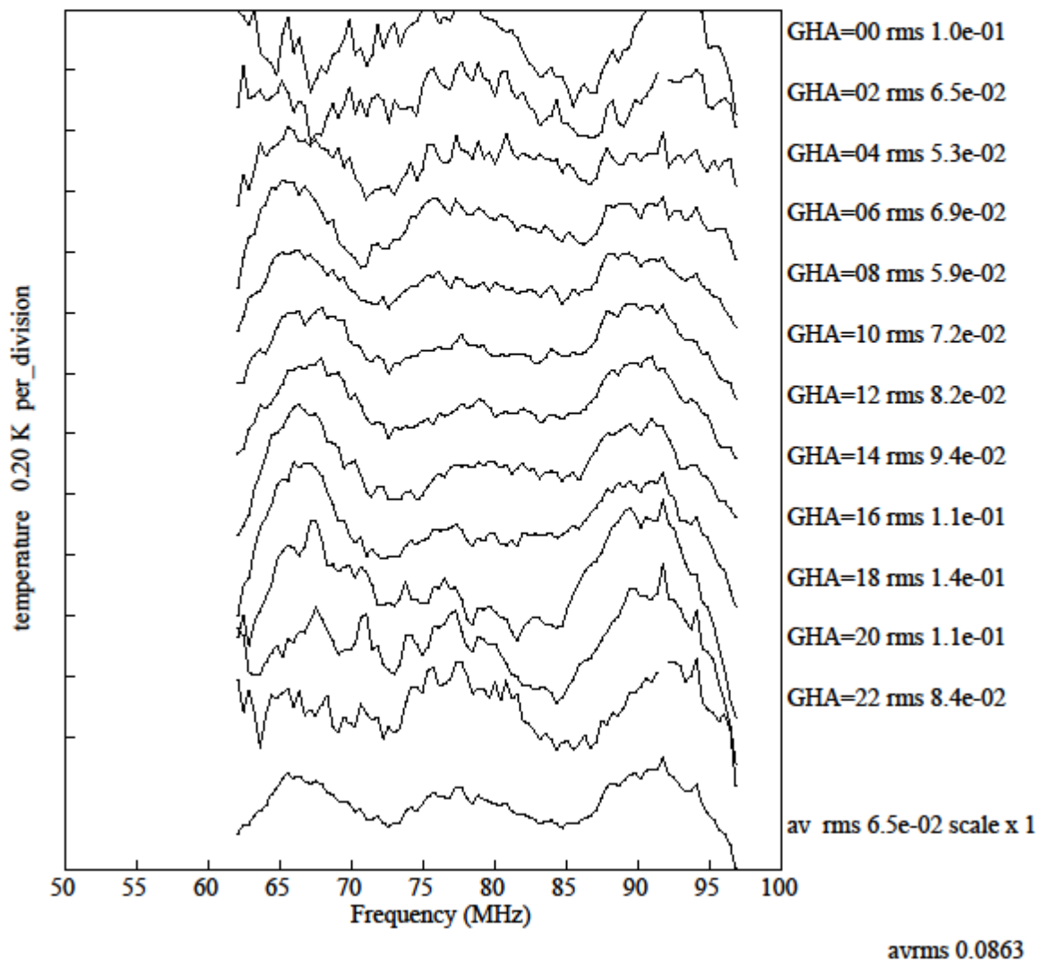
Figure 4. Lowband1 residuals with 4 polynomial terms removed.
