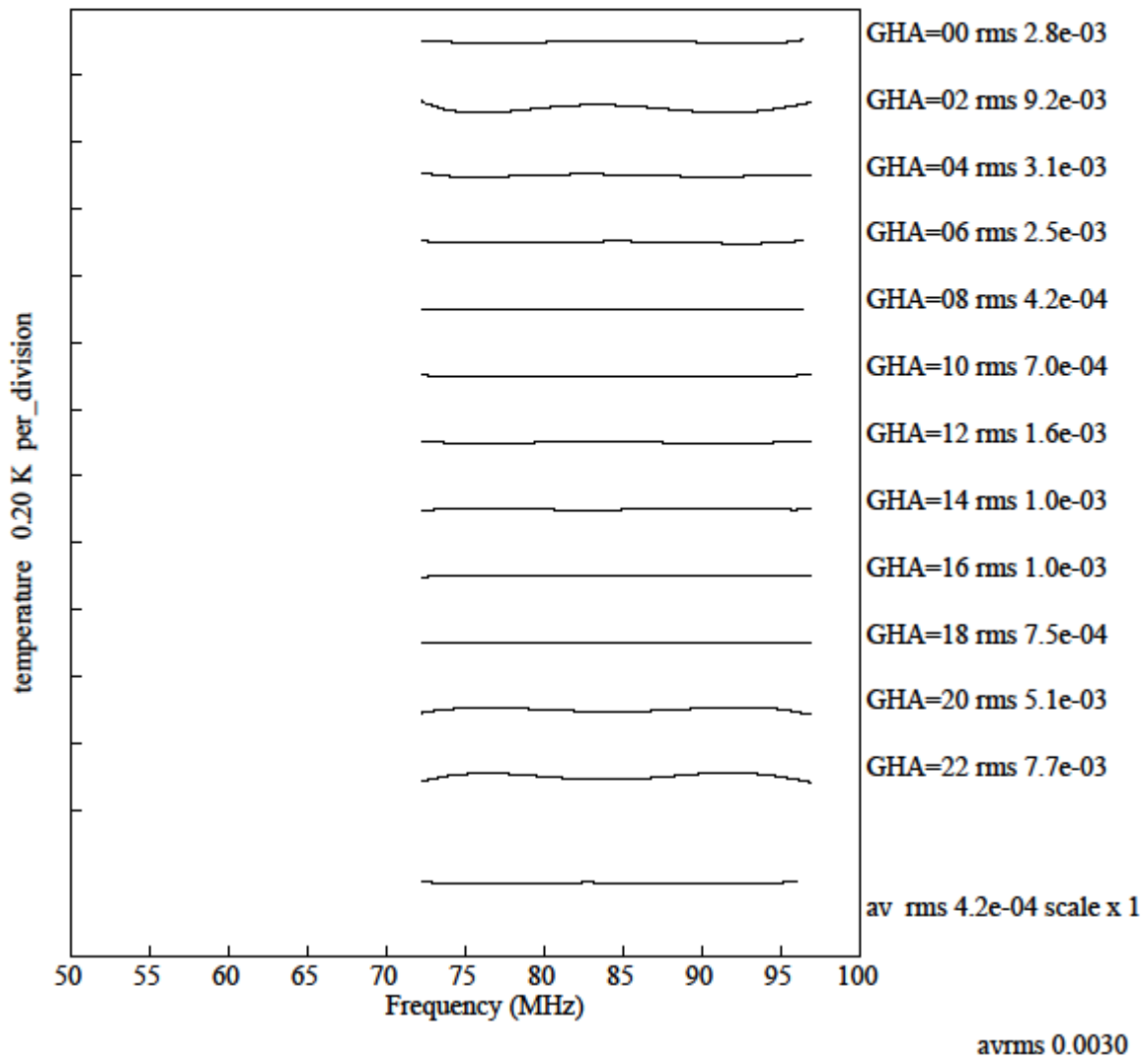
Figure 2a. Simulated residuals for change in soil with 4 term polynomial removed.
