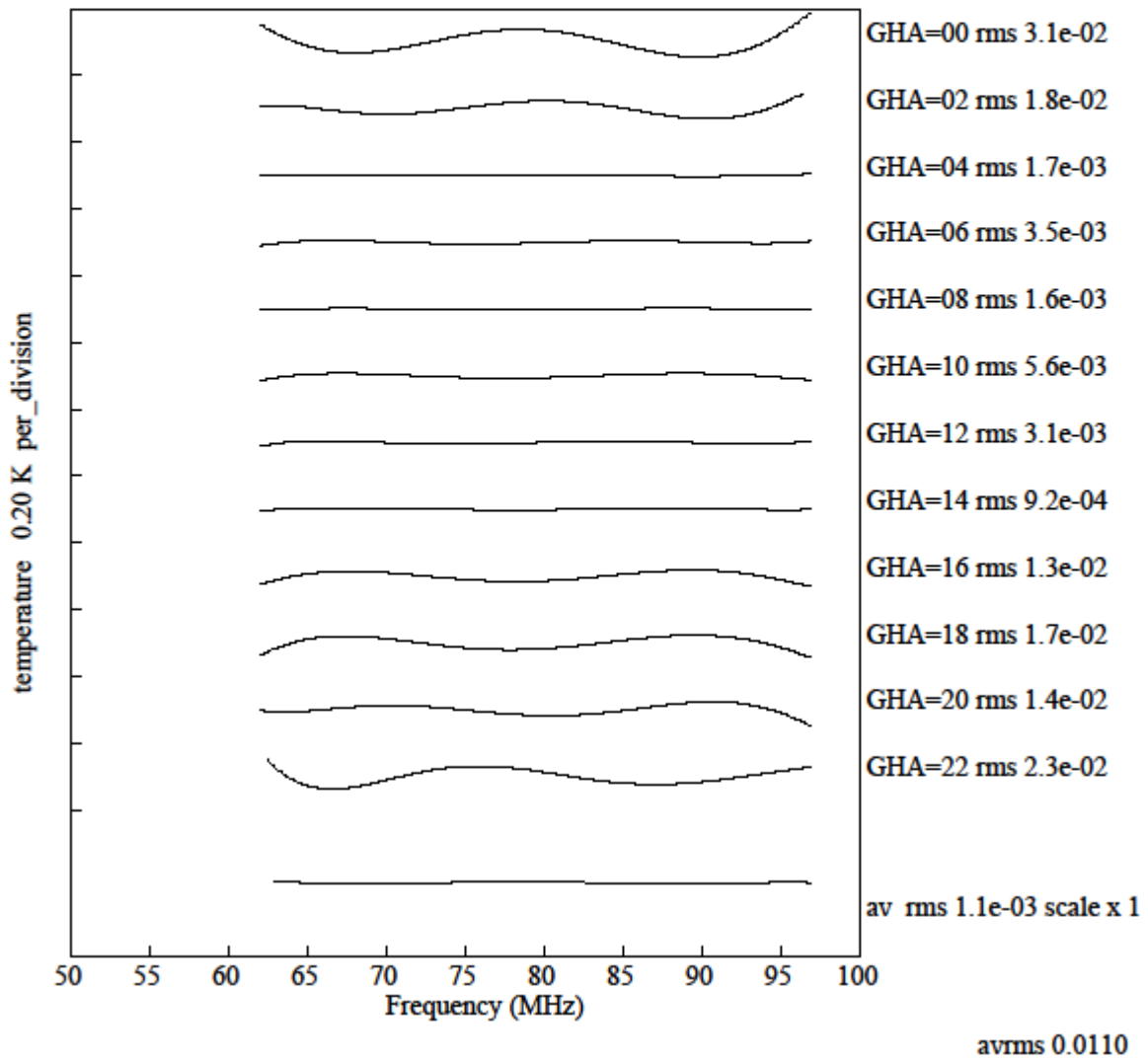
Figure 2b. Effects over larger frequency range.
