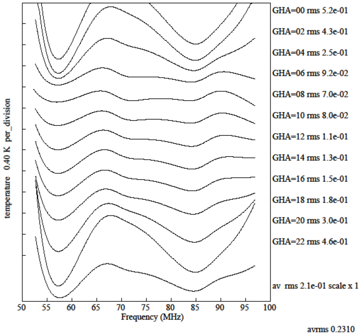
Figure 7. Simulation with added signature as in Figure 5 over larger frequency range for comparison with lowband1 data residuals shown in Figure 5.
