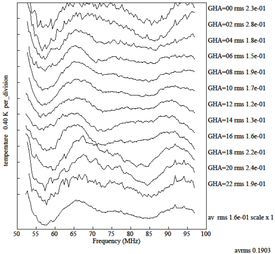
Figure 6. Lowband1 data residuals with 4 polynomial terms removed.
