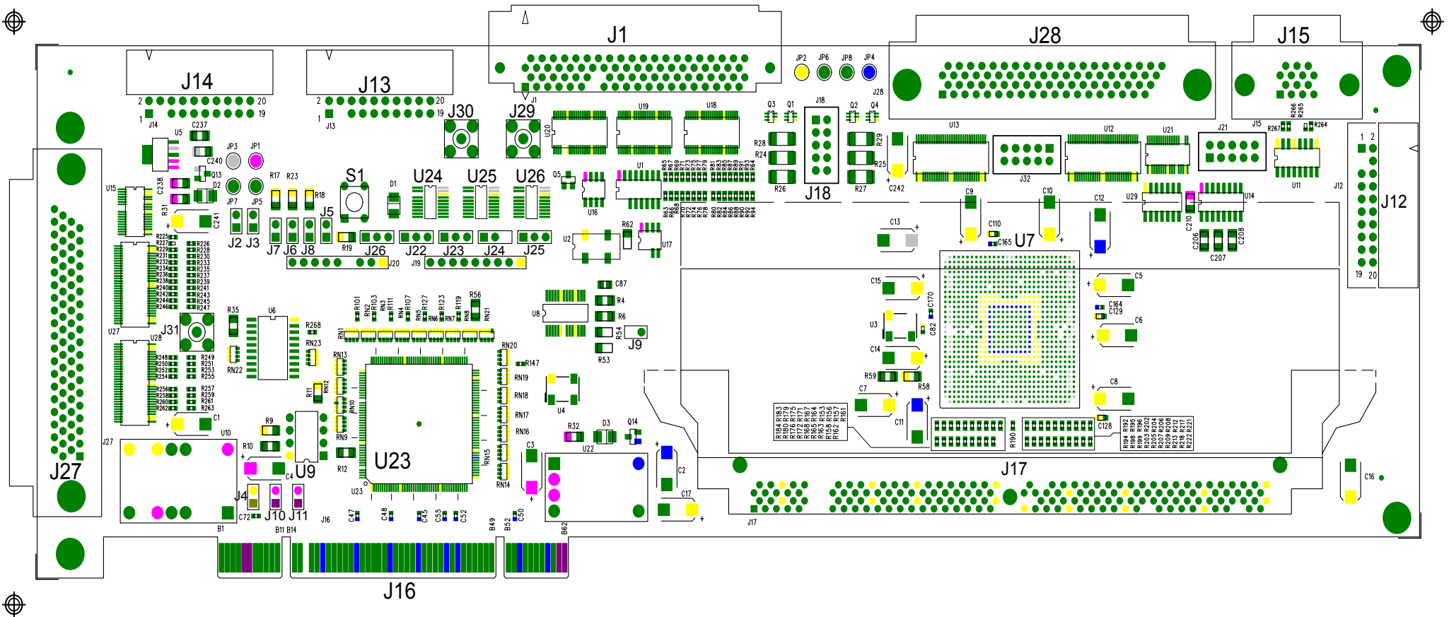
FIGURE 1 MARK 5B I/O BOARD
