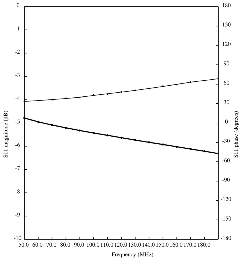
Figure 2. Reflection coefficient of “hot filament” source. Lower curve is the phase.
