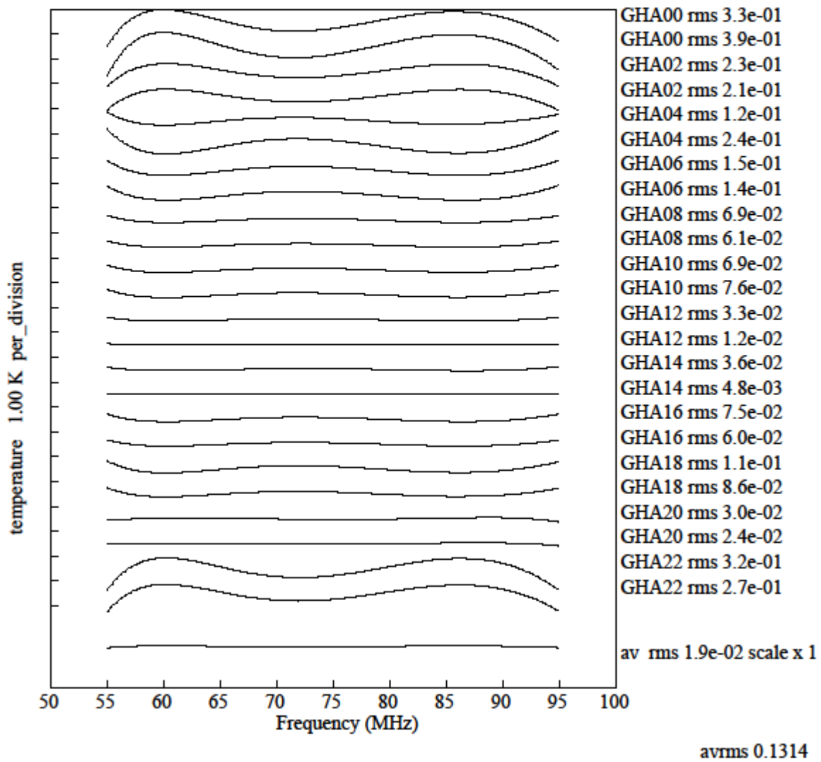
Figure 1. Simulated residuals to beam corrections using 4 polynomial fit for an infinite ground plane at the MRO.
