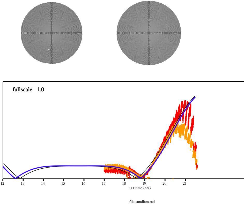
Figure 2 is a plot of the interferometer correlation amplitude vs UT for 31 October (in red) and 1 November (in orange). Also shown on the figure are curves for the expected amplitude for a uniform disk on 0.54 degrees diameter* (in black) and for a uniform dish of 0.56 (in blue). Clearly the larger diameter is the better fit which shows that the Sun appears to be about 12% larger than the optical disk at 12 GHz.
