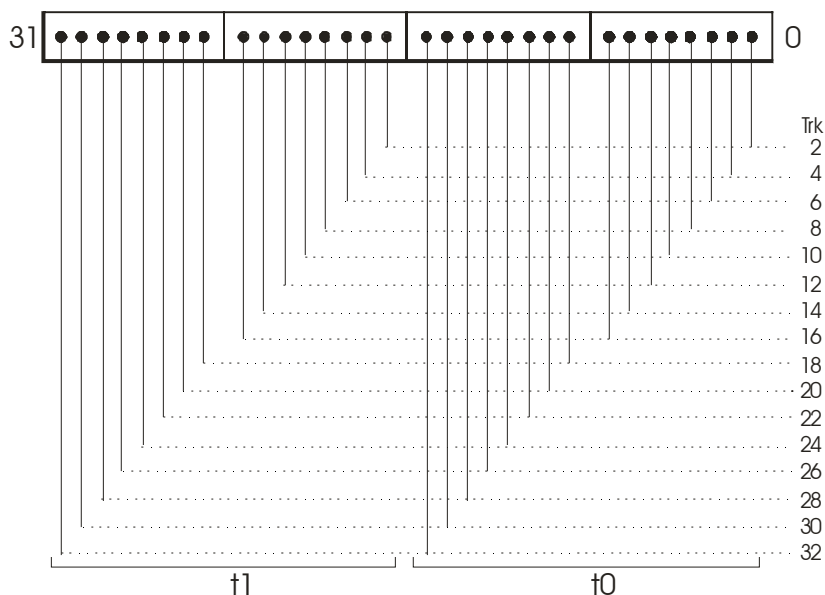
Figure 2: Mapping of bits in FPDP word to tracks for all cases of 16 output tracks. Output track groups will be duplicated in the same manner as Mark 5A. t_0 – t_1 refer to output-track clock cycles.
