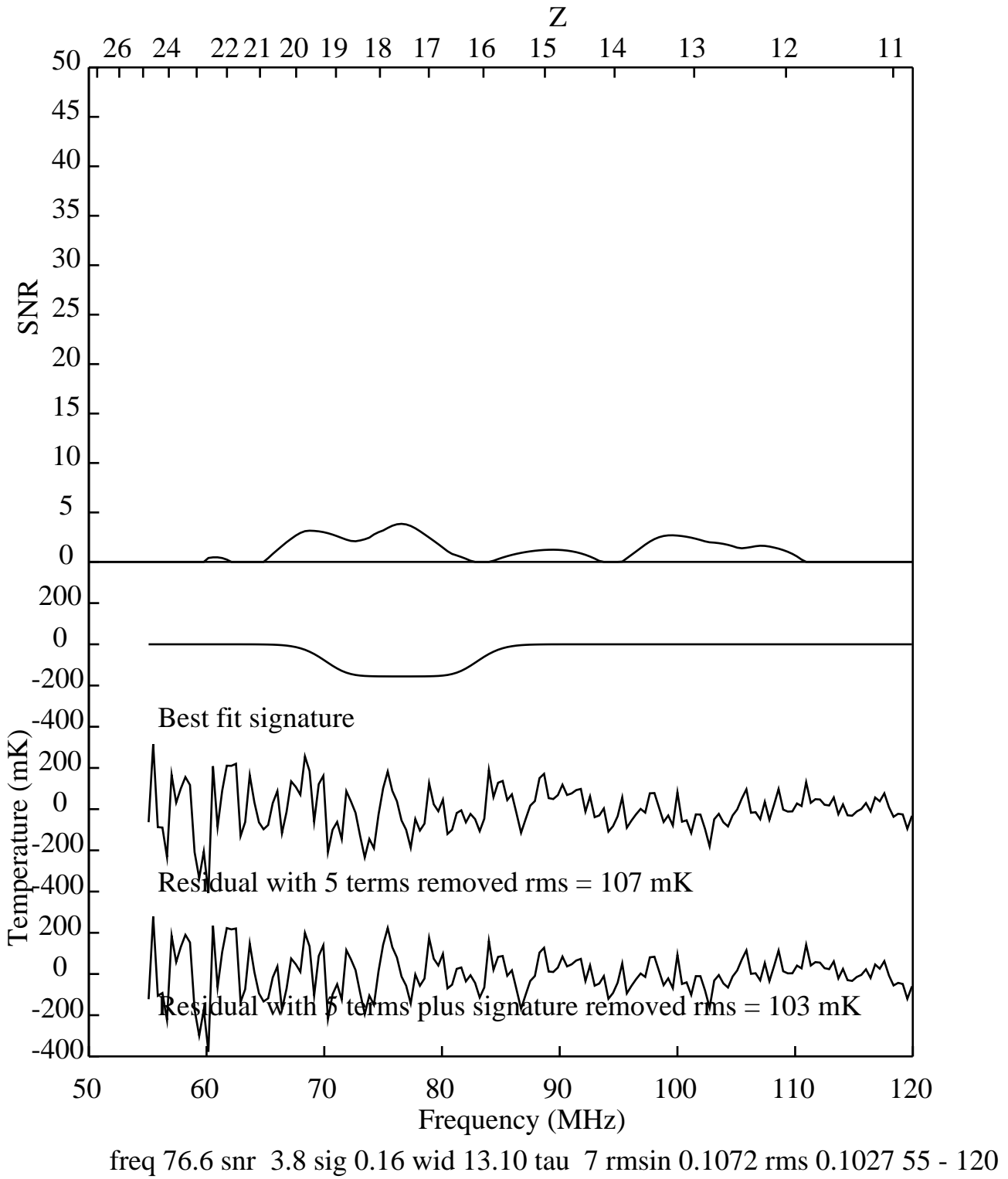
Figure 3. Feature search of 48 hour integration on the artificial antenna simulator.
