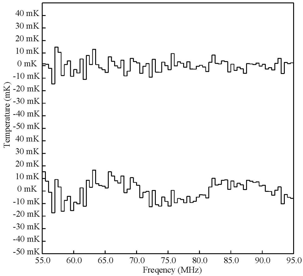
Figure 4. The lower curve shows the residuals to the best fit using basis functions 0 through 7 while upper curve shows the residuals for the best fit which includes basis function 8. This shows that the 100 mK absorption is not completely removed by the basis functions needed to remove the foreground, ionosphere and frequency dependence of the beam.
