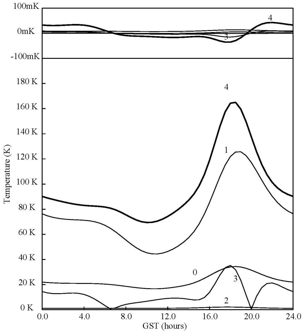
Figure 3. Same as figure 2 for a latitude of 42 degrees. For both latitudes the performance is slightly better with the dipole oriented NS.
