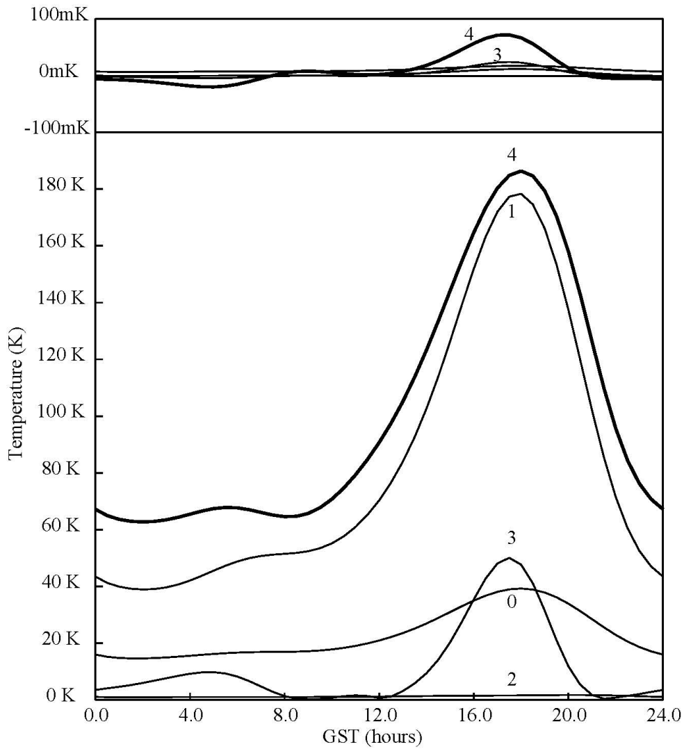
Figure 2. Lower curves are same as in figure 1. Upper curves are the values of EoR signature bias introduced by the lack of ability of the basis functions to accommodate the deviations of the foreground from an ideal uniform spectral index of -2.5 . The curves labeled 3 and 4 are for the effect of the antenna beam variation and all effects combined respectively.
