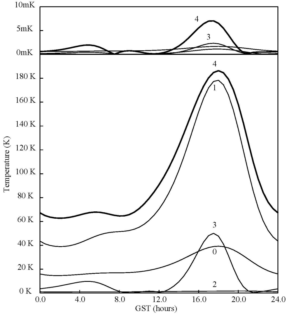
Figure 1. Lower curves are the rms deviations from a nominal spectral index of -2.5 for the ionosphere, spectral index, ionospheric refraction and frequency dependence of the beam and all combined labeled 0, 1, 2, 3, 4 respectively. The upper plot are the rms deviations after removing the 8 basis function.
