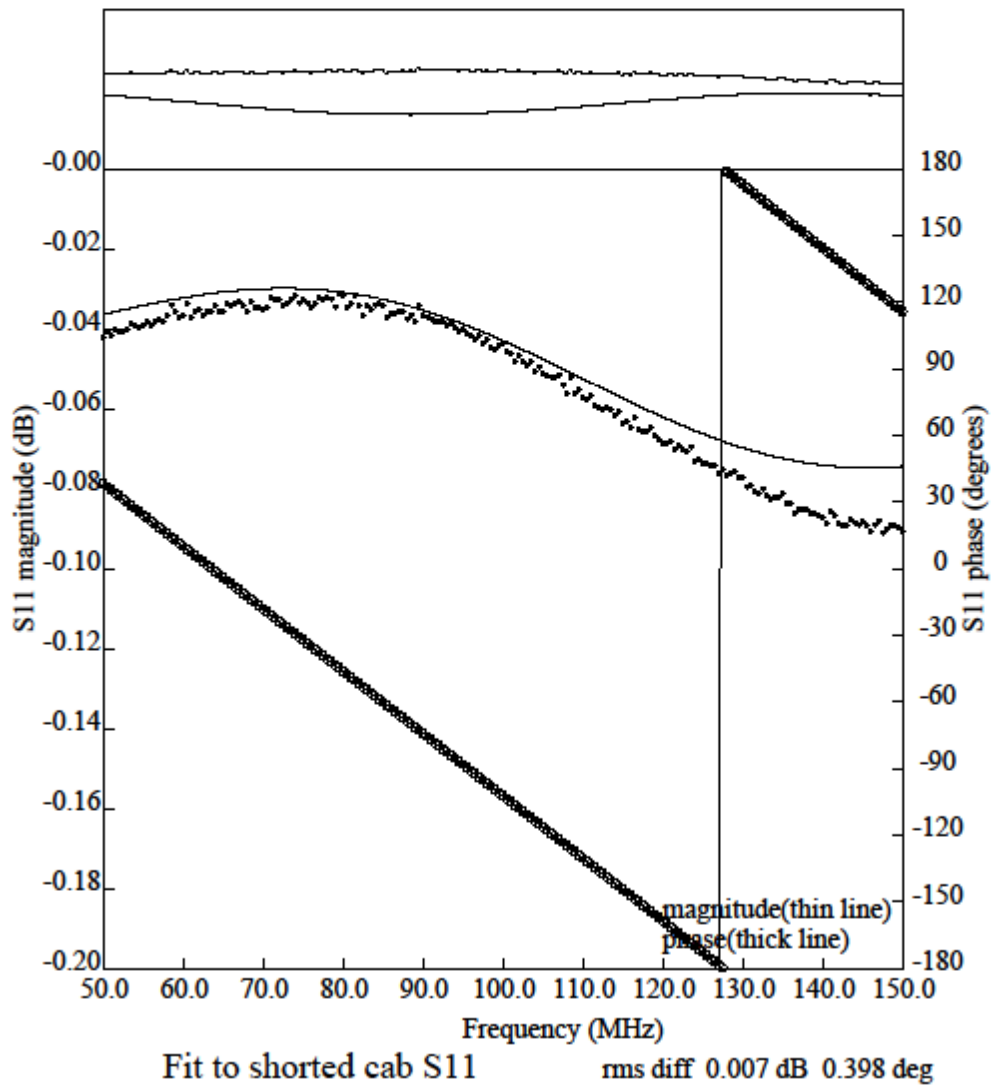
Figure 2. Comparison of S11 with model with shorted end.
