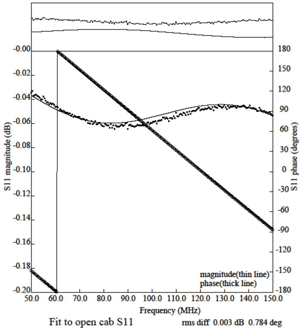
Figure 1. Comparison of S11 with model for open ended low band balun.
