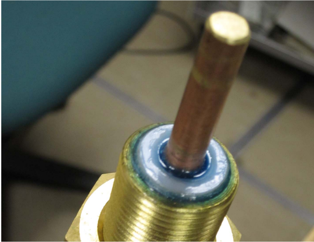
Figure 3. Balun center conductor bonded to balun tube using LORD 305-1/2 epoxy.
