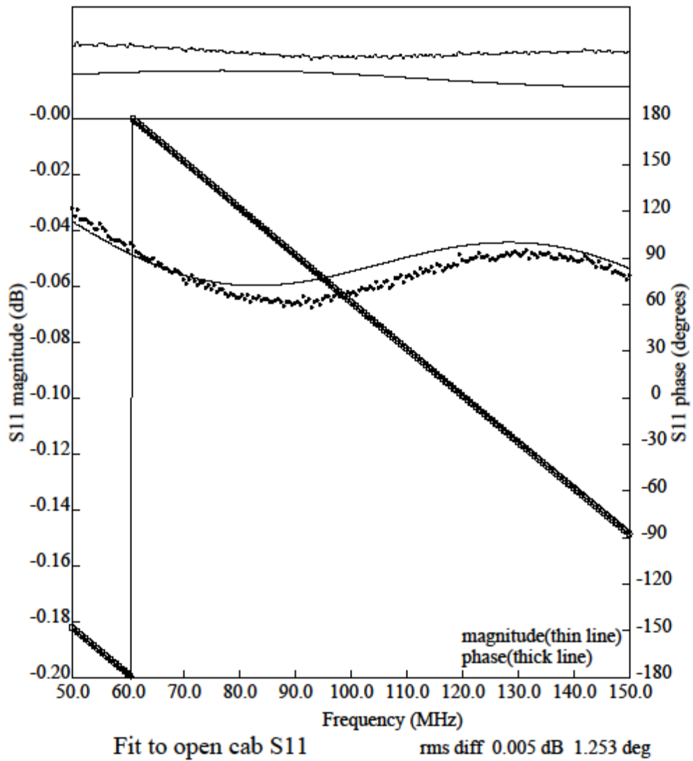
Figure 6. Balun S11 measured with open end.
