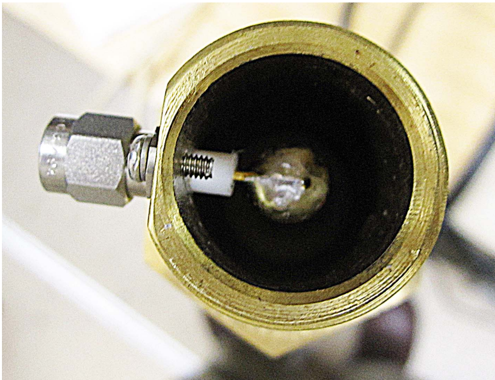
Figure 4. Center conductor soldered to Fairchild microwave SC3792 SMA male connector shown with polystyrene plug removed.
