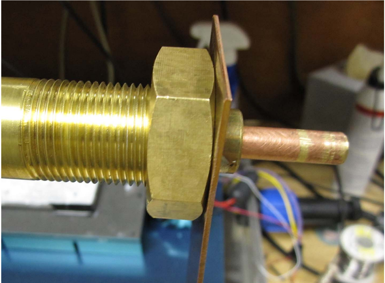
Figure 8. Balun end shorted with nut tightened against top cap.
