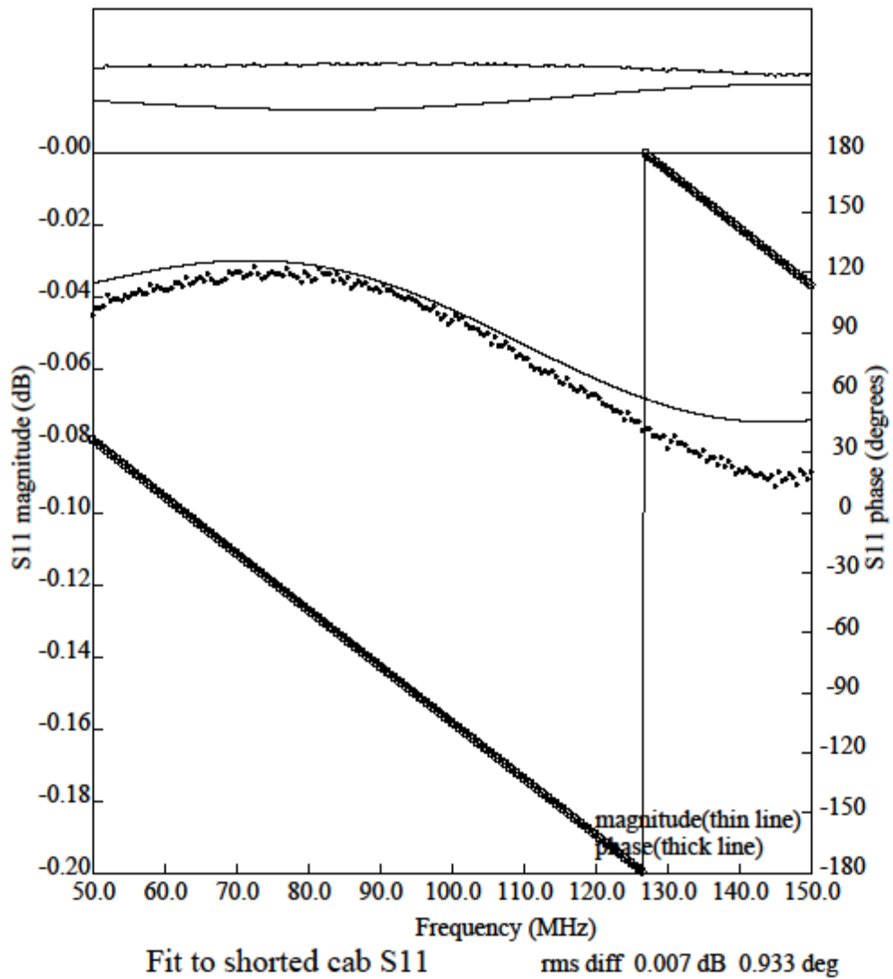
Figure 7. Balun S11 measured with short shown in Figure 8.
