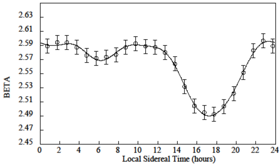
Figure 6. Spectral index for nighttime data from high band using 2-term fit.
