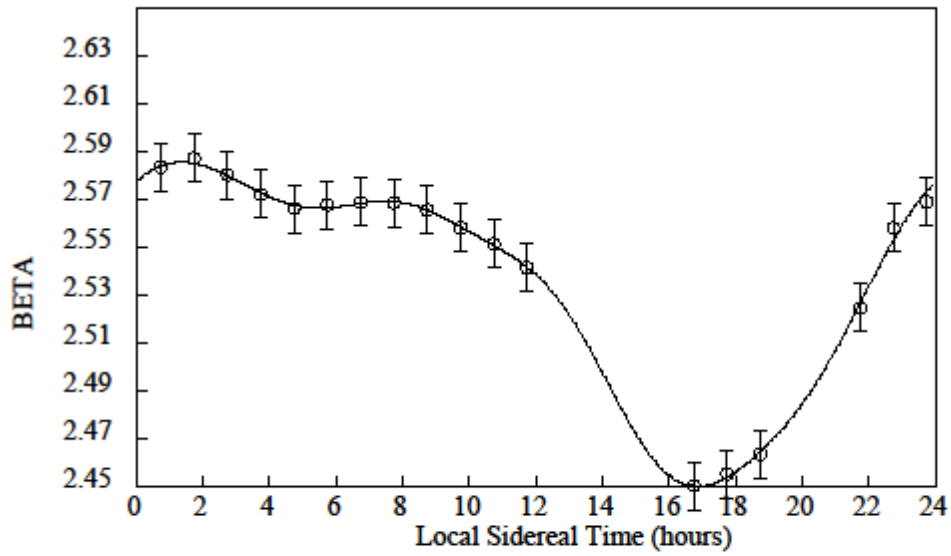
Figure 5. Spectral index for nighttime data from low bands using 2-term fit.
