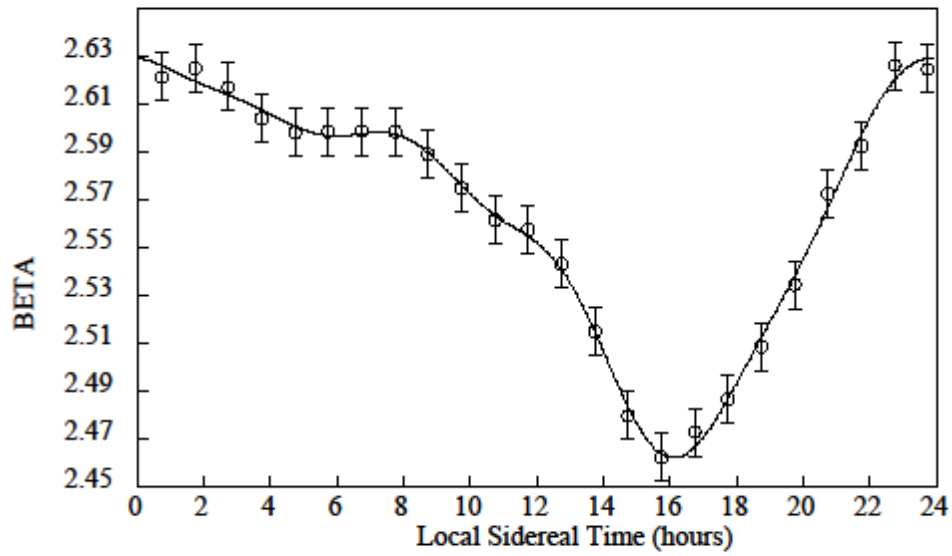
Figure 7. Spectral index from low band using 3-term fit.
