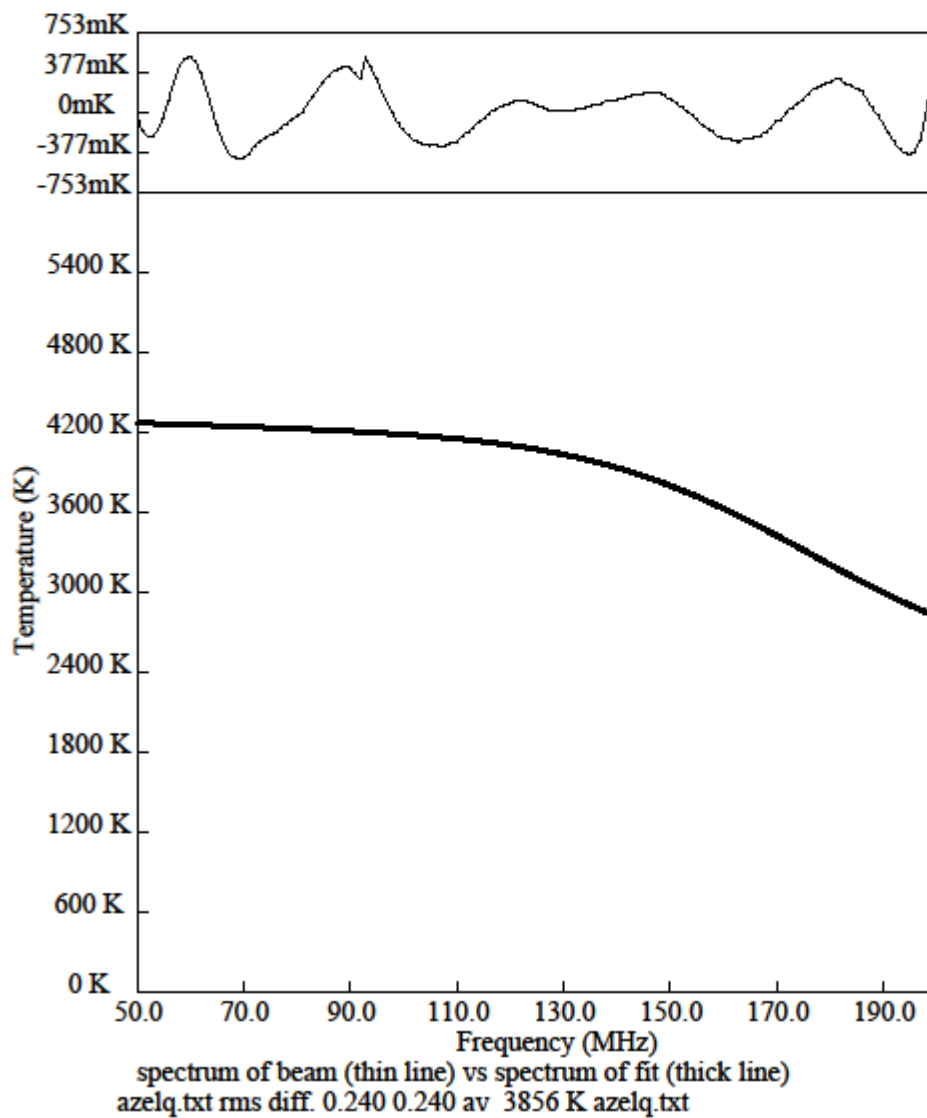
Figure 1 Glitch in FEKO beam calculation at 92 MHz shown in residuals to 9-term polynomial fit to beam corrections.
