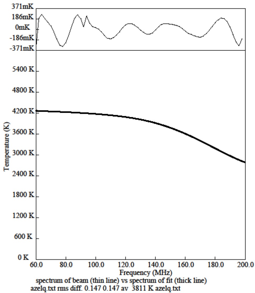
Figure 2. Similar glitch in separate FEKO processing.
