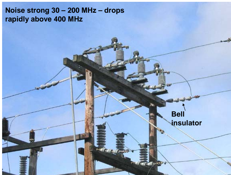
Noise strong 30 – 200 MHz – drops rapidly above 400 MHz Power line noise causes: leaking insulators, poor connection on “slack span”, microarcing in bell insulators. See Power-Line Noise Mitigation Handbook for Naval and Other Receiving Sites @ www.arri.org
